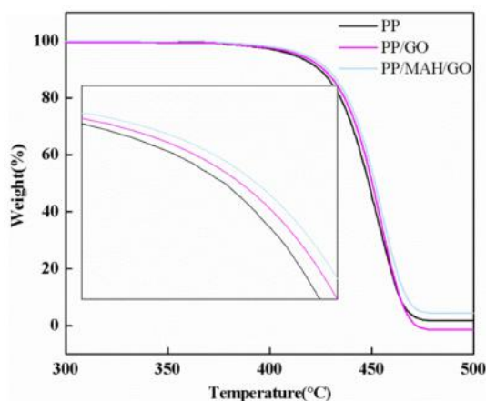
Figure 5. TGA image of composite fibers.
